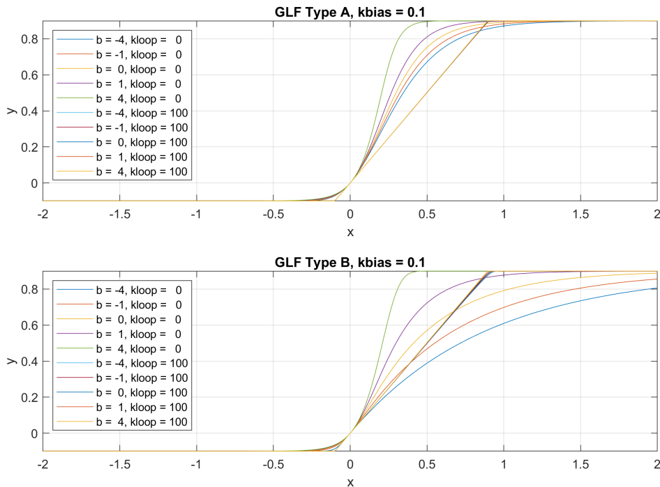
Fig. 7: The generalized logistic functions for k_{\text{bias}} = 0.1
